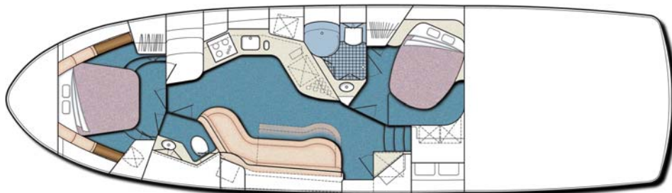
Cabin Layout
